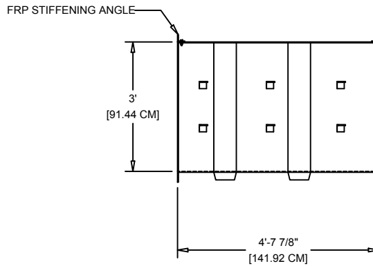
ELEVATION VIEW
